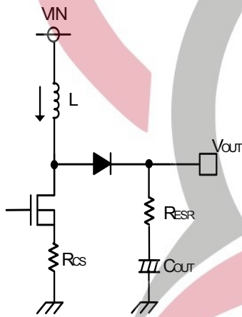
Figure 25. Output part
